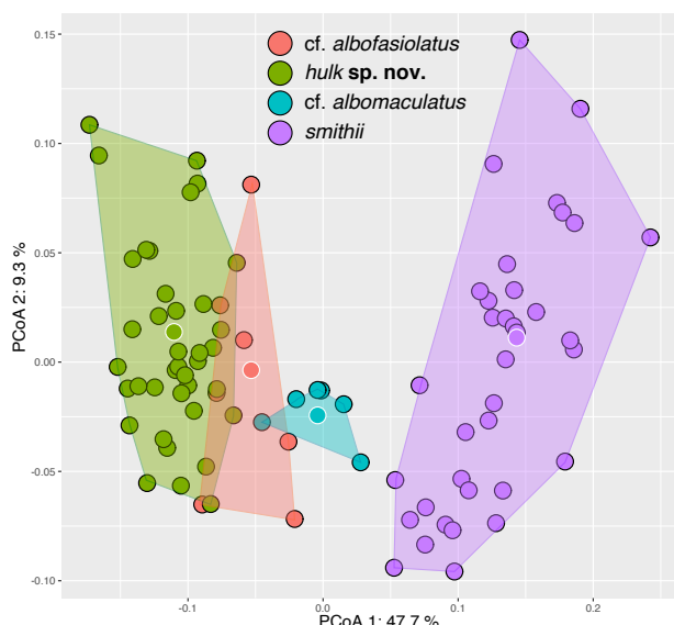
Figure 4. PCoA of concatenated meristic and morphometric data of species of the Gekko smithii complex.
